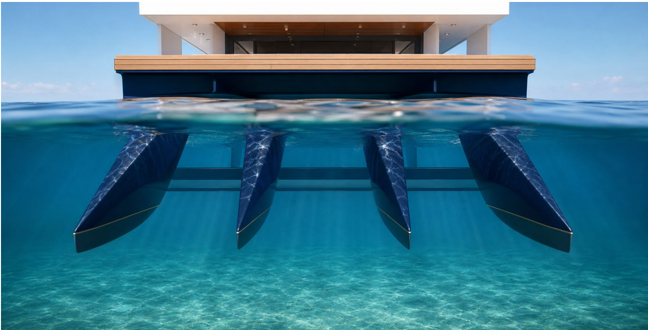
Quadrimaran platform, split waterline — four parallel hulls and the transverse tunnel structure that ties them. Concept render.
